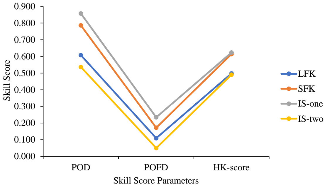
Figure 4.5: Skill Scores of LFK, SFK, IS-one and IS-two
